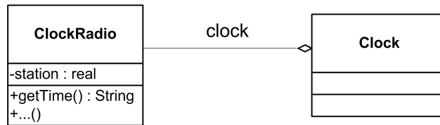
Figura 20: Simulation of inheritance of Clock by ClockRadio
