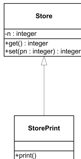
Figura 10: UML representation of Store and StorePrint
