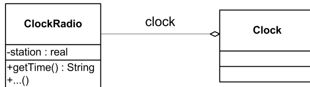
Figura 20: Simulation of inheritance of Clock by ClockRadio
