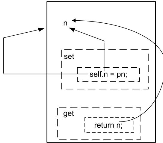
Figura 3: References to self in object s
